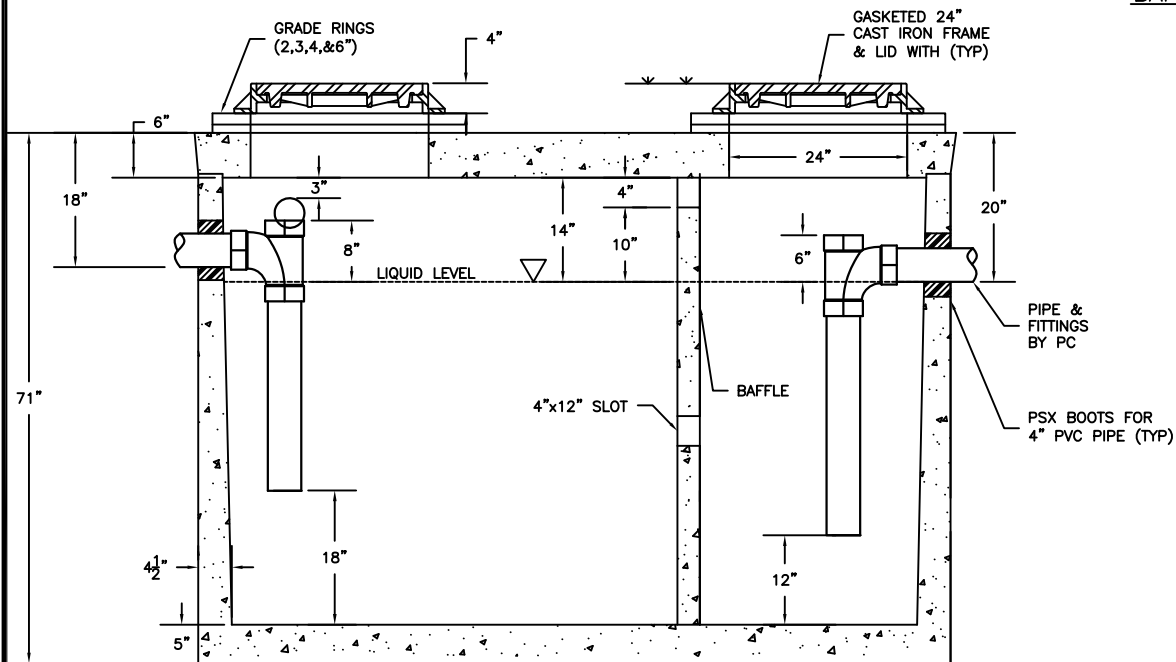
SECTION VIEW
